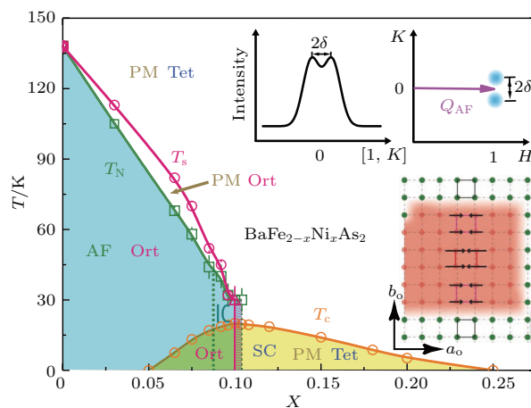
图 4 电子型掺杂 \text{BaFe}_{2-x}\text{Ni}_x\text{As}_2 的相图 [47], 插图为非公度反铁磁序和自旋玻璃态的示意图 Fig. 4. Phase diagram for electron-doped \text{BaFe}_{2-x}\text{Ni}_x\text{As}_2 [47]. The inset shows the schematic of incommensurate AFM Bragg peak and spin glass state.
