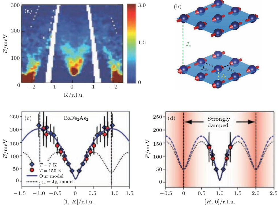
图5 (a)BaFe 2 As 2 的自旋波谱; (b) 磁交换耦合作用的示意图; (c)[1,K] 方向的自旋波分布,其中实线和虚线是海森伯模型拟合的结果,分别对应的是面内各向异性和各向同性的磁交换耦合常数; (d)[H,0] 方向的自旋波分布 [54] Fig. 5. (a) Spin wave in BaFe 2 As 2 ; (b) the schematic of magnetic exchange couplings; (c) spin-wave dispersion curves and fits using a Heisenberg Hamiltonian with different exchange couplings along the [1,K] direction; (d) similar Heisenberg Hamiltonian fits along the [H,0] direction [54] .
