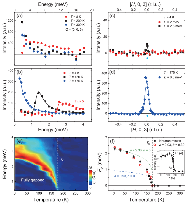
Figure 4 (Color online) (a) Energy dependence of the spin excitations at T = 8, 200, and 300 K measured at Taipan. (b) High resolution energy dependence of the spin excitations at T = 4, 150, and 175 K measured at Sika. (c), (d) Constant-energy scans for E = 2 and 2.5 meV at T = 4 K, and E = 0.3 meV at T = 175 K. The solid lines are Gaussian fittings, and the horizontal bars indicate the instrument resolution. (e) Temperature dependence of the spin dynamic susceptibility \chi''(Q, \omega) at low energy. (f) Temperature dependence of the spin wave gap and fitting results by eq. (2) with different parameters. Inset shows the integral intensity \chi''(\omega) up to 4 meV.
