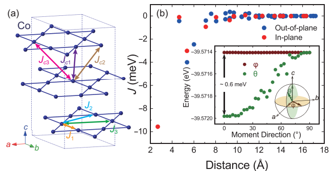
Figure 3 (Color online) (a) Effective exchange interactions between Co atoms in our first principle calculations. (b) Estimation of the effective correlation length of the exchange interactions (main panel) and the total energy of the moment rotation (inset) for both in-plane and out-of-plane cases.
