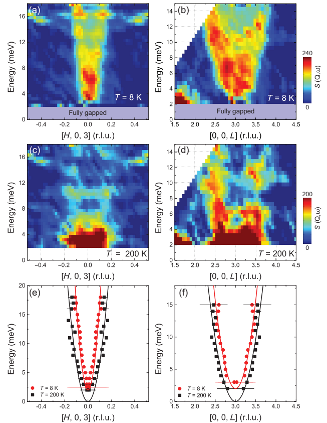
Figure 2 (Color online) (a)-(d) In-plane and out-of-plane spin waves at T = 8 K and paramagnetic excitations at T = 200 K around Q = (0, 0, 3) . The high energy data at low Q side in panel (c) and (d) are missing due to scattering restrictions, and strong contaminations from quasi-elastic scattering prevent measurements of data below 2 meV. (e), (f) Dispersion of the spin excitations obtained from two Gaussian-fittings of the raw data. The solids lines are fitting results with q^2 -dependence.
